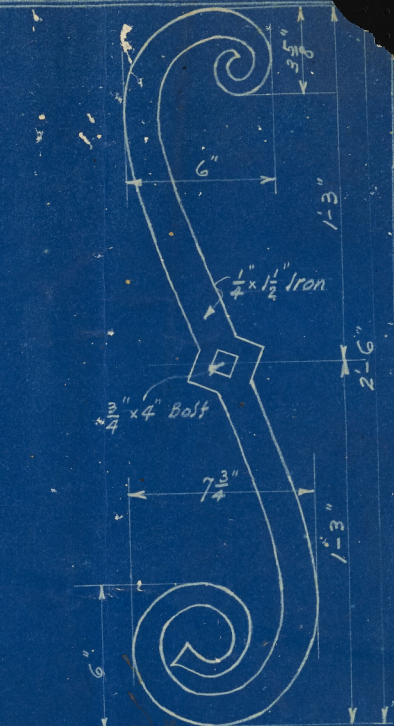
3" SC. DET. of CHIMNEY ANCHOR
