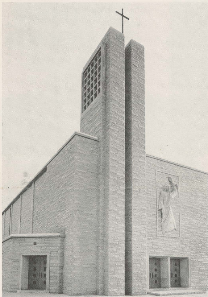
This modern church is the St. Barnabas Church, Philadelphia, Pennsylvania. It is faced with Mount Airy Sawed Bed Ashlar, Pattern #2, medium rise. Architect B. W. Roney has obtained permanence as well as a pleasing effect. The stone was placed by F. Cantono & Sons, and the General Contractor was J. R. Farrell, Inc.
