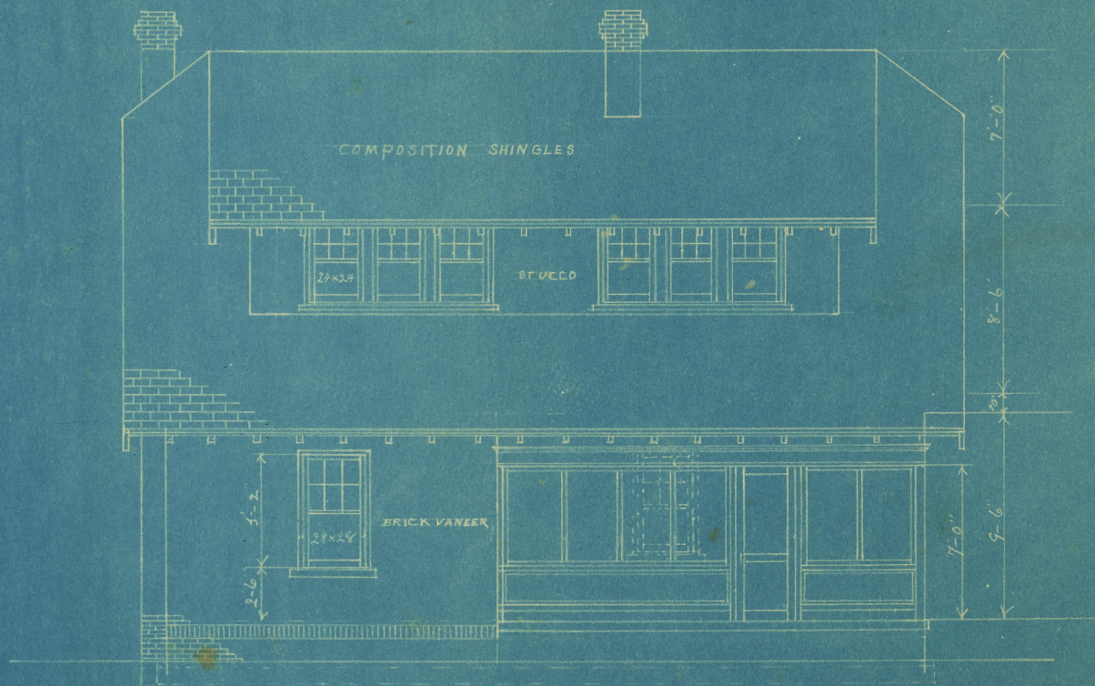
REAR ELEVATION, SCALE \frac{1}{4}" = 1'
